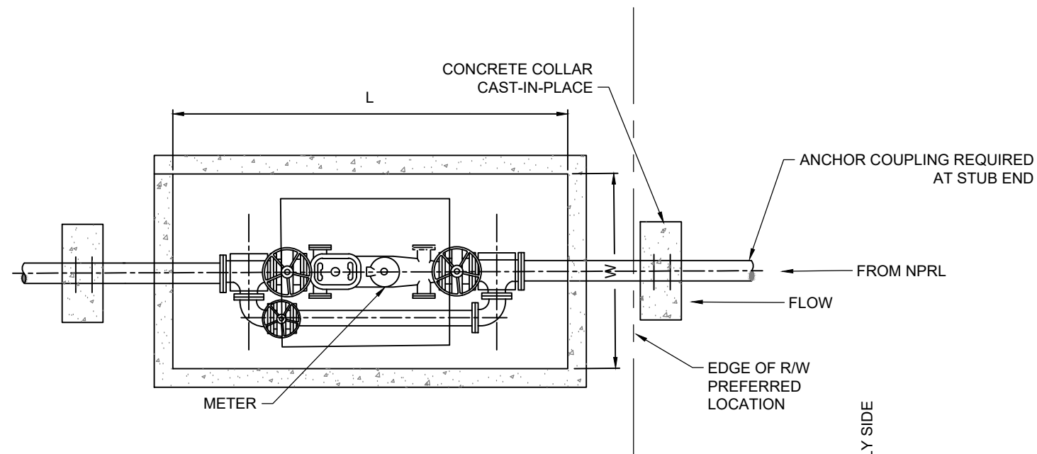
VAULT PLAN VIEW
