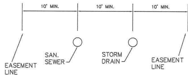
N.T.S. TYPICAL COMBINATION SAN. SEWER AND STORM DRAIN PERMANENT EASEMENT
